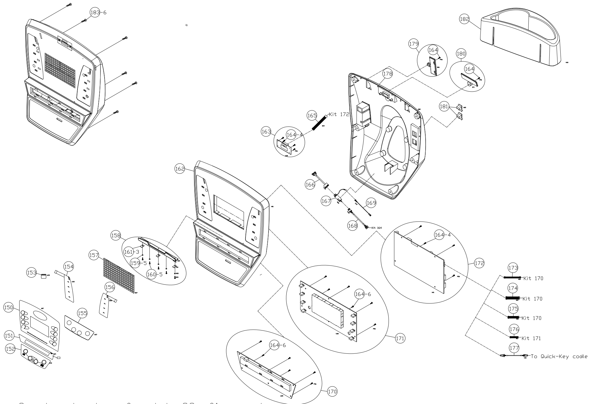
Service drawing of matrix S3x-01 console
